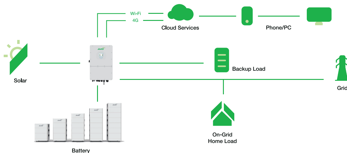
JinKo's RESS system diagram
